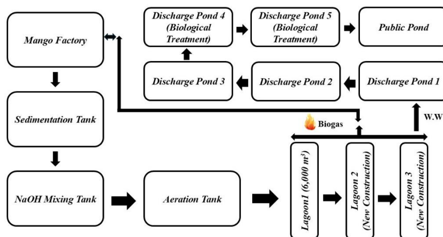
Fig. 1 Diagram of wastewater treatment at the mango processing factory
